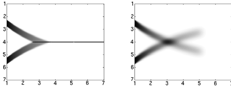
Fig. 2. Simulation of crossing jets with drag and evaporation at time t = 10 using the multi-fluid model (left) and the multi-fluid multi-velocity model (right).
